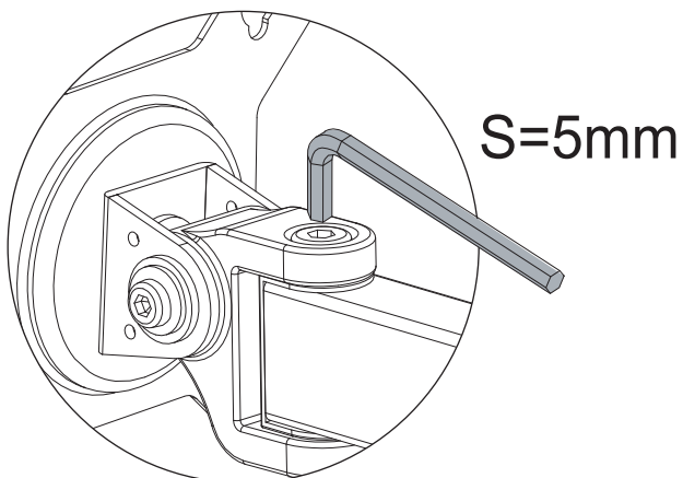
VESA Swivel Adjustment
